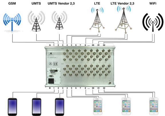
(fig. 6. Handover test setup)
