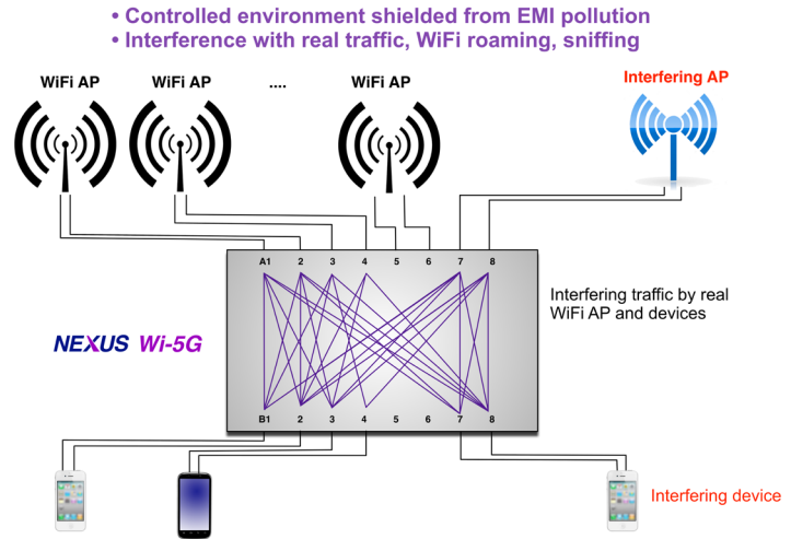
(fig. 8. Carrier WiFi testing)
